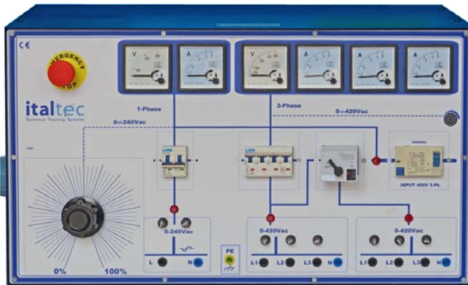
- Mod.3002 3-Ph/1Ph AC power supply 3+3A
